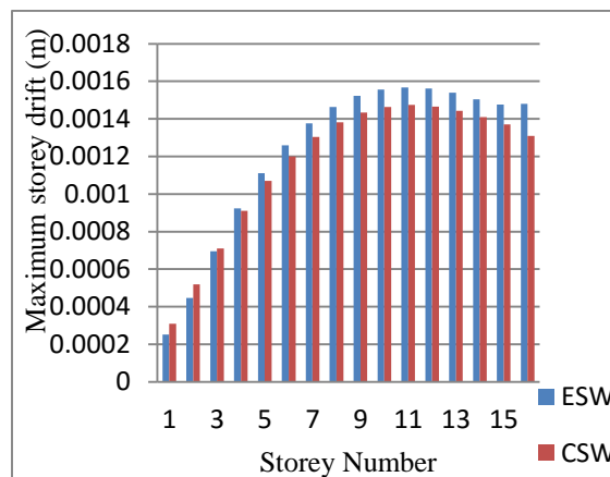
Fig 10: Maximum storey drift in Seismic ZONE – III
