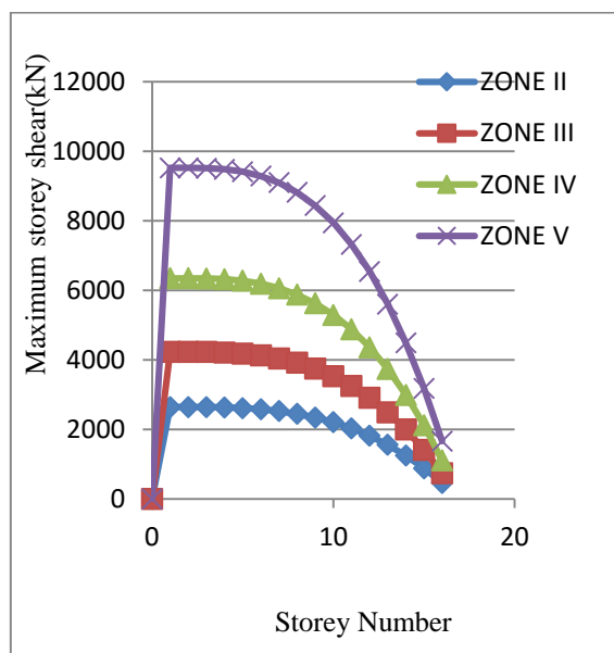
Fig 26: comparison of storey shear (kN) in all earthquake zones for edge shear wall
