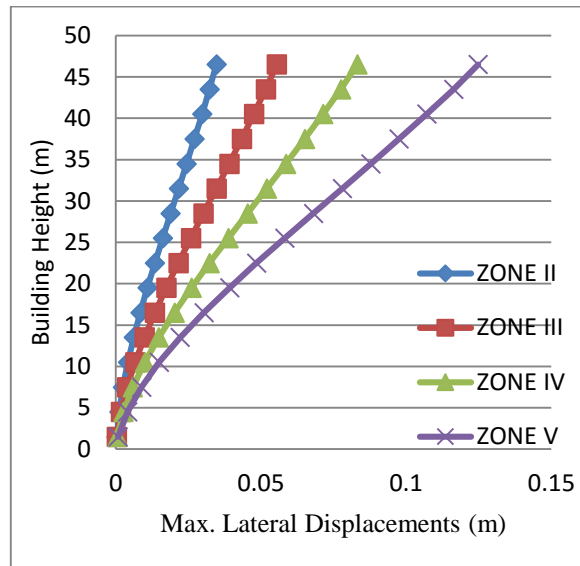
Fig 20: distribution of lateral storey displacements (m) along the height of building in all earthquake zones for CSW model
