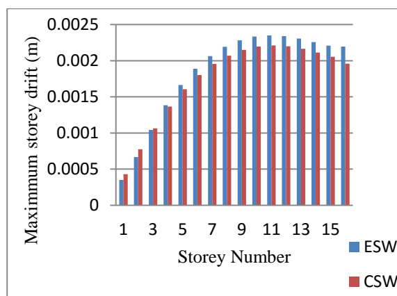
Fig 11: Maximum storey drift in Seismic ZONE – IV
