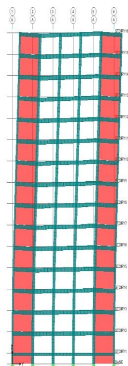
Fig 8: Deformed shape of G+14 storey ESW model in y-direction
