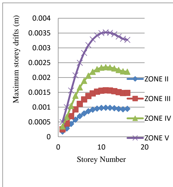
Fig 13: comparison of storey drifts (m) in all earthquake zones for Edge shear wall model
