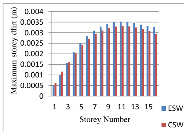
Fig 12: Maximum storey drift in Seismic ZONE – V
