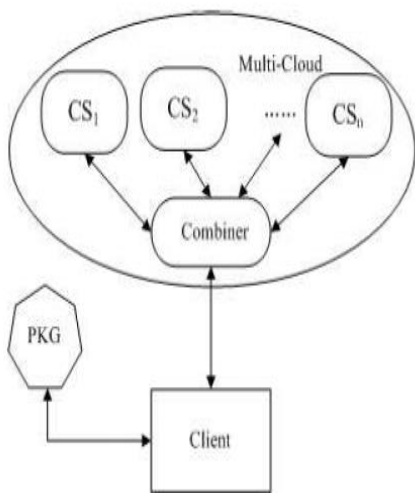
Fig. 1. The System Model of ID-DPDP
